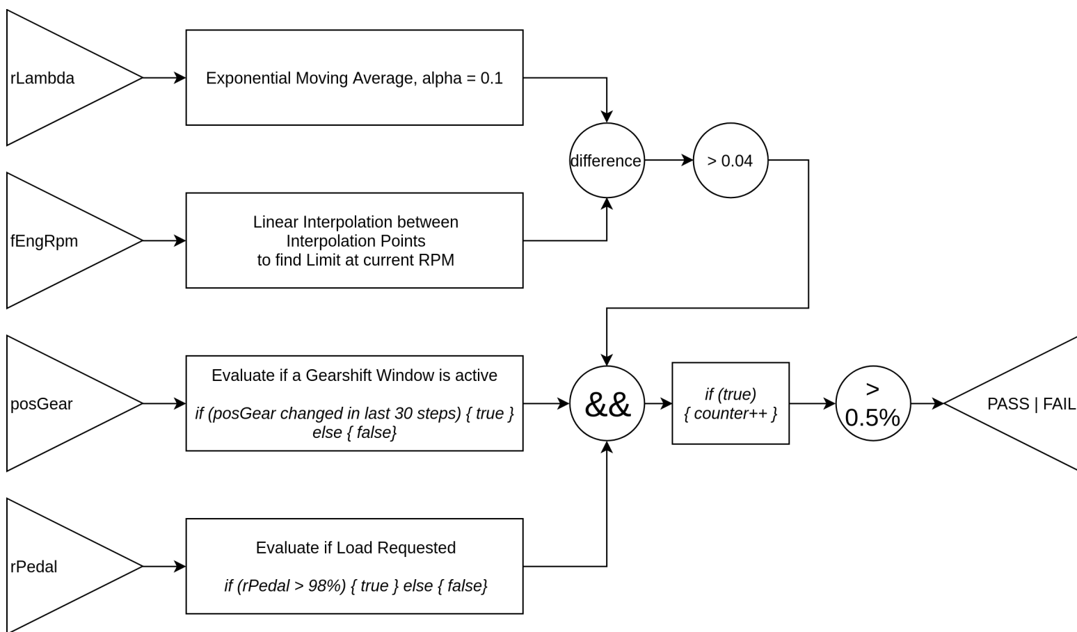
Figure 1: Lambda Monitoring Method Block Diagram
